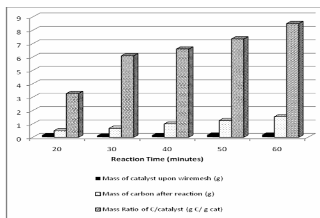
Figure 5. Carbon yield at various reaction times.
