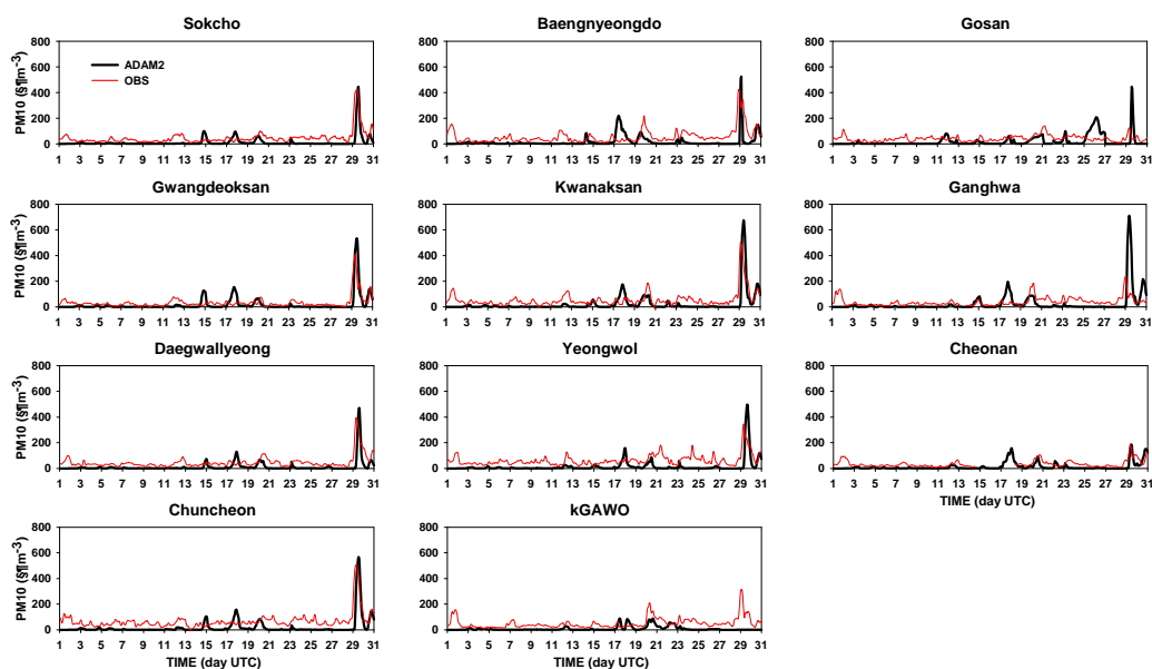
Figure 11. Time series of observed (—, red) and modeled (ADAM2(—)) surface PM_{10} concentration ( \mu g m^{-3} ) at the downstream sites in Korea in December 2007.
