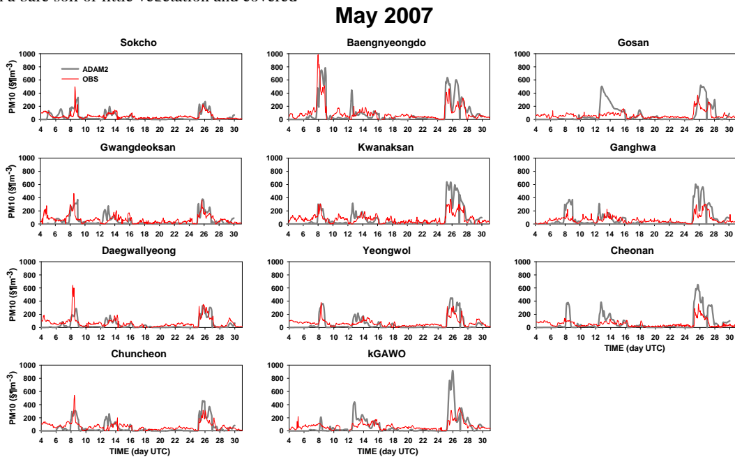
Figure 6. Time series of observed (—, red) and modeled (ADAM2(—)) surface PM 10 concentration (µg m -3 ) at the downstream sites in Korea in May 2007.
